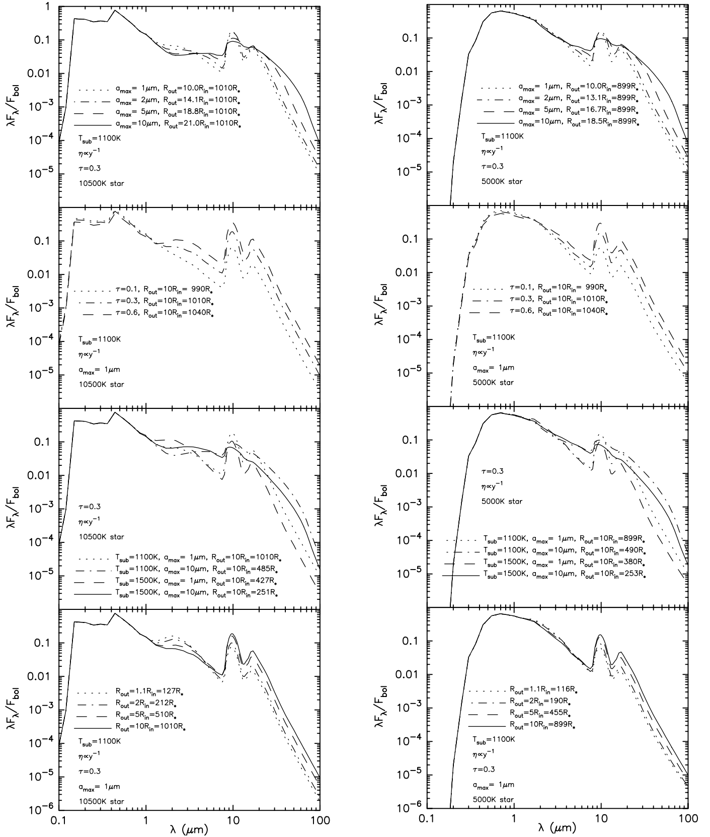
FIG. 5.—SED variation with the parameters of small spherical halos around stars with 10,500 and 5000 K (Kurucz stellar models). The radial density profile is \eta \propto r^{-1} . The dust chemistry is x = 0.4 olivine from Dorschner et al. (1995). The grain size distribution is n(a) \propto a^{-2} between minimum grain radius 0.01 \mu\text{m} and maximum a_{\text{max}} , as marked. The other varied parameters are the dust sublimation temperature T_{\text{sub}} , which sets the halo inner radius R_{\text{in}} , the halo outer radius R_{\text{out}} and its optical depth at visual \tau . Note the variation of R_{\text{in}} among models, especially when a_{\text{max}} is increased.
